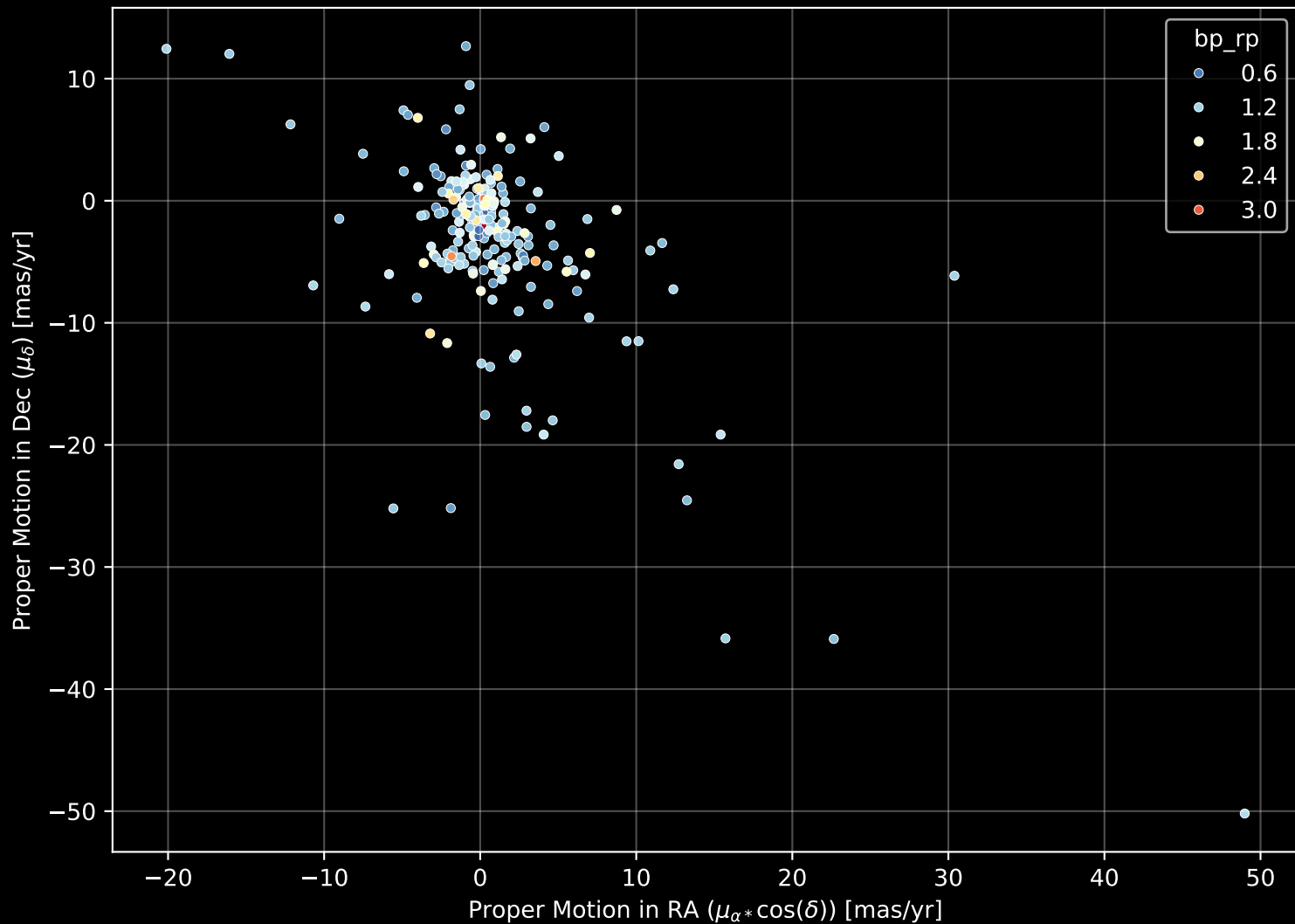
GALAH DR4 Field: [9272] Proper Motion Diagram (n= 231)
