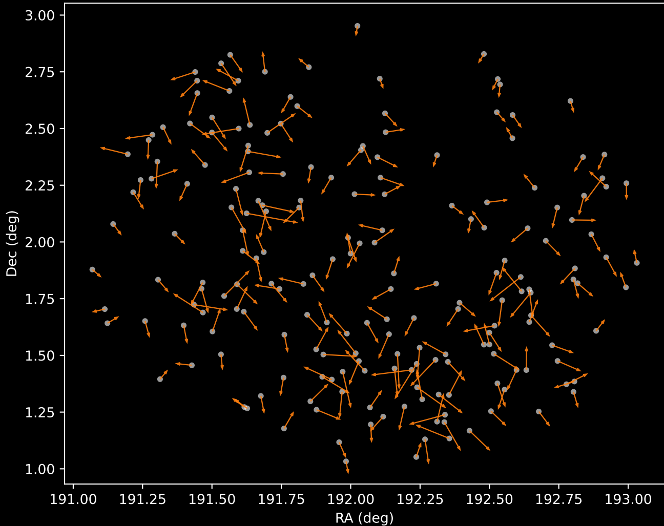
GALAH DR4 Cluster 2 Proper Motion Vectors (n=196)
