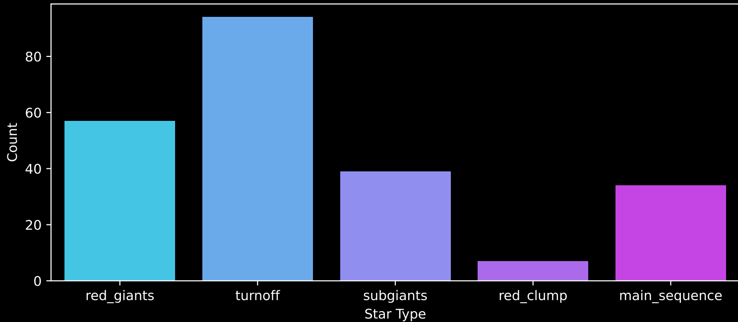
GALAH DR4 Field: [9272] Count plot of Star Type
