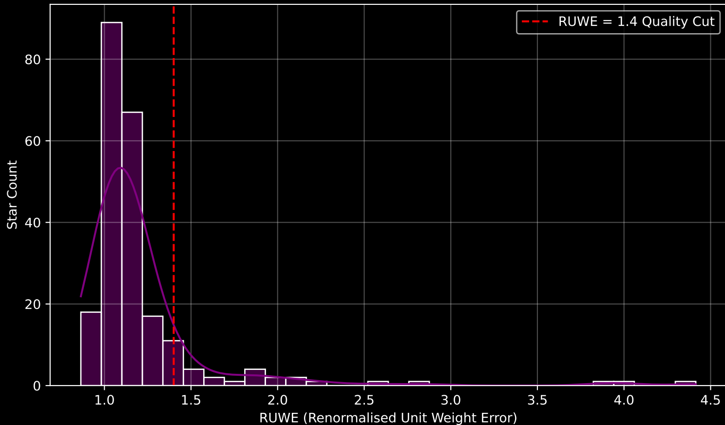
GALAH DR4 Field [9272] RUWE Distribution (n= 223)
